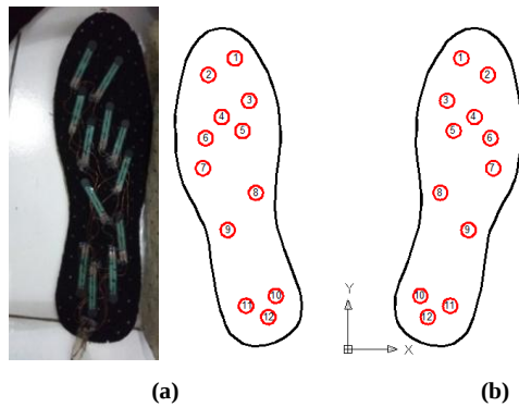
Figure 3: (a) Simple Insole for Dynamic Foot Plantar Measurement; (b) Location FSR placement
