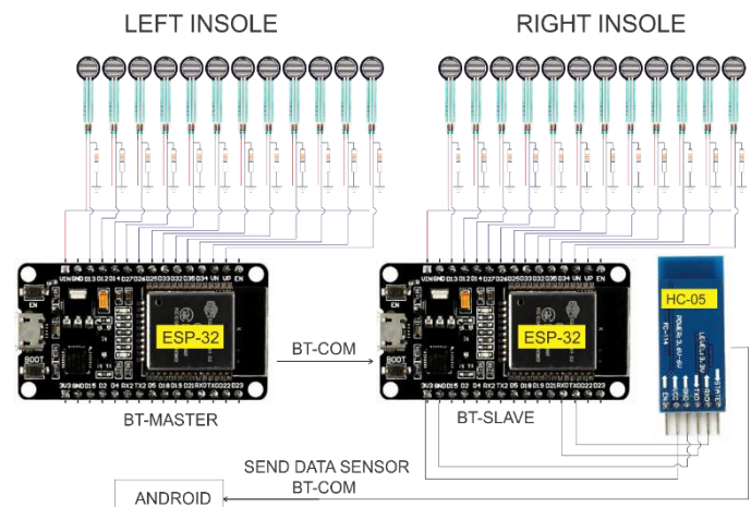
Figure 2: Hardware Design
