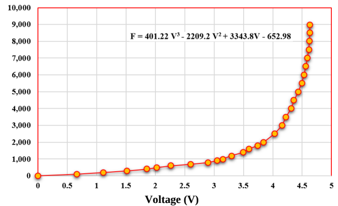
Figure 1: Relationship between Load (gram) and Voltage (V)
