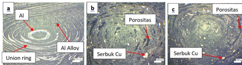
Gambar 8. Distribusi Partikel Cu pada Overlap ( Metallography Optic )
