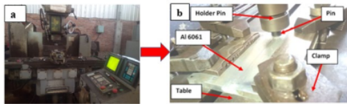
Gambar 4. a), Universal Milling Machine, b) Schematic FSW
