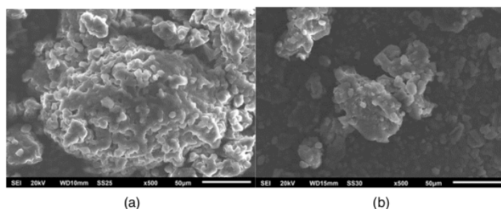
Fig. 3 - SEM micrograph of; (a) pretreated magnified 500 X, and (b) raw winged bean flour magnified 500X
