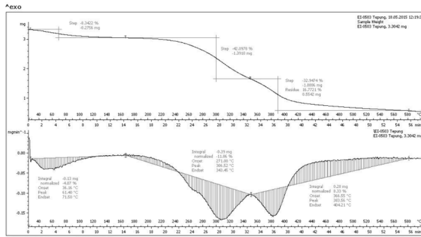
Fig. 1 - TG and DTG of pretreated winged bean flour at flowrate 200 ml/minute, rate 10°C/min
