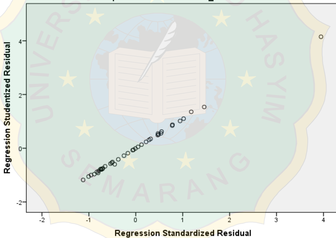
Scatterplot
